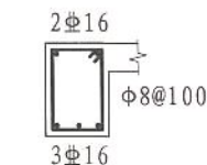
TL3 280 × 400
