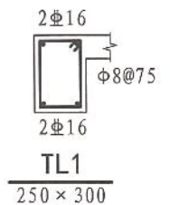
TL1 250 × 300
